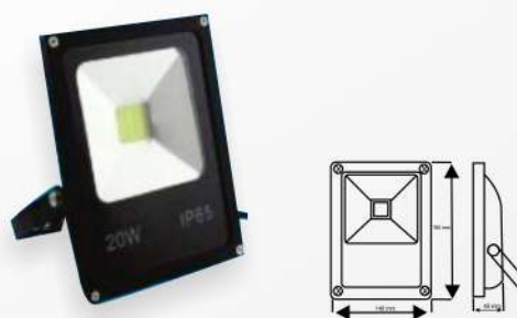
DIMENSION (mm)
