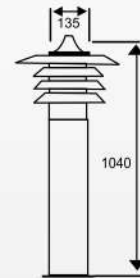
DIMENSION (mm)
