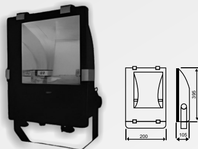
W FL MHN-TD 70-150W H 494 LC
