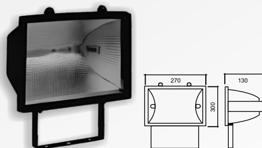
W FL Halogen 1000W H 495 LC
