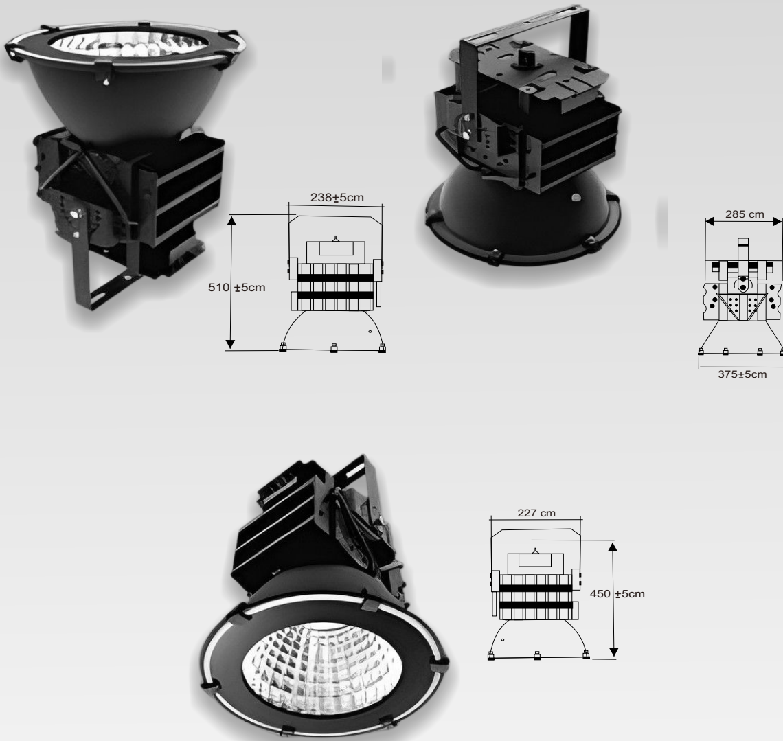
W FLB LED 300W H 4112 LC
