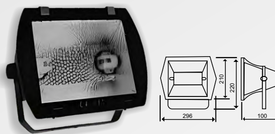
W FL MHN-TD 70-150W H 493 LC
